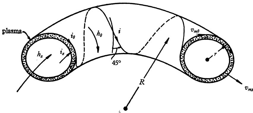
Fig. 1. The S-plasmoid . This configuration of magnetic field and plasma is essentially the same as that of the H-centered pinch in a toroidal tube which was first proposed and investigated experimentally in the United States in 1955 by M. A. Levine and L. S. Combes [Tufts University, Dept. of Physics Report, January 30, 1956 (unpublished)]. The configuration has since received theoretical development by M. N. Rosenbluth and C. L. Longmire [ Annals of Physics , 1 , 120, 1957]. Papers 47-49 of this volume are reports on experimental and theoretical work on the same configuration in a straight tube (see also I. N. Golovin et al. , J. Atomic Energy U.S.S.R. , 5 , 26, 1956; V. D. Shafranov, J. Atomic Energy U.S.S.R. , 5 , 38, 1956).
